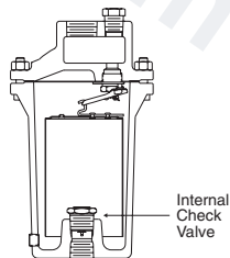
Fig. 19-3. Internal check valve installed in trap inlet of 200 Series trap.
