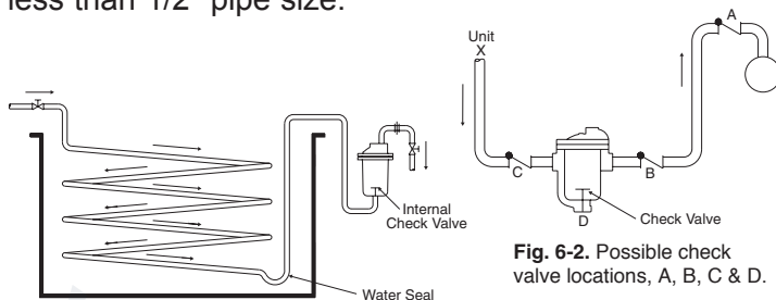
Fig. 6-1. Trap draining syphon.
