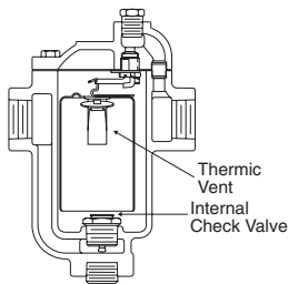
Fig. 19-2. Internal check valve installed in trap inlet.
