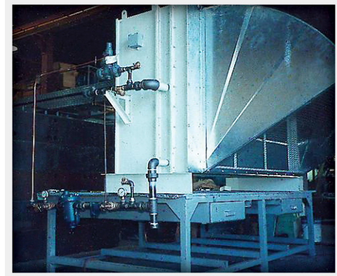
Make-Up Air Package with Posi-Pressure, Control System, and Rainhood
