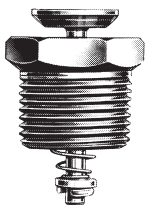
Fig. 18-2. Armstrong stainless steel internal check valve.
