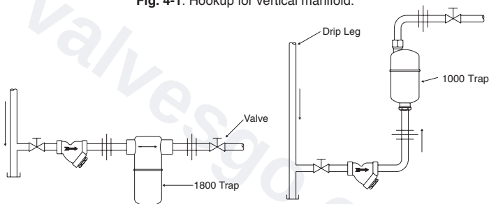
Fig. 4-2. Hookup for No. 1800 Series Stainless Steel trap.
