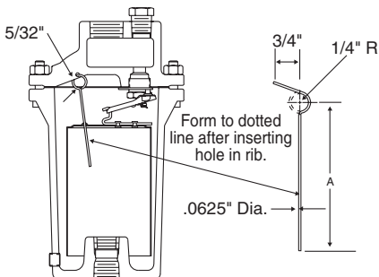
Fig. 16-1. Vent scrubbing wire for use when oil plugs vent. Trap inlet tube must be removed.
