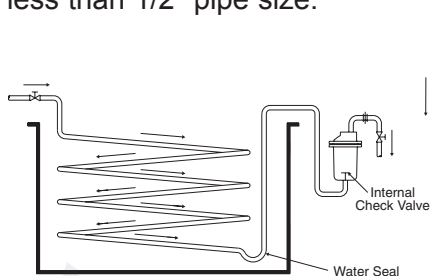
Fig. 6-1. Trap draining syphon.
