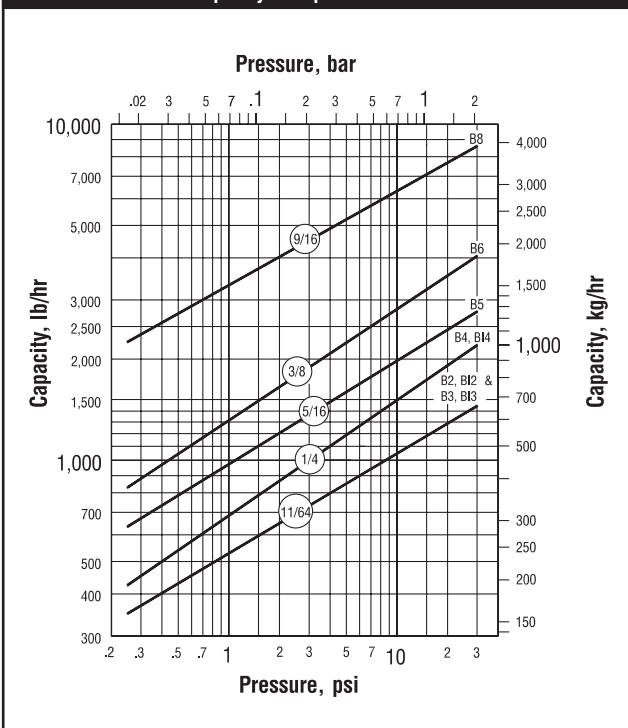
Model B & BI Series Capacity—30 psi
