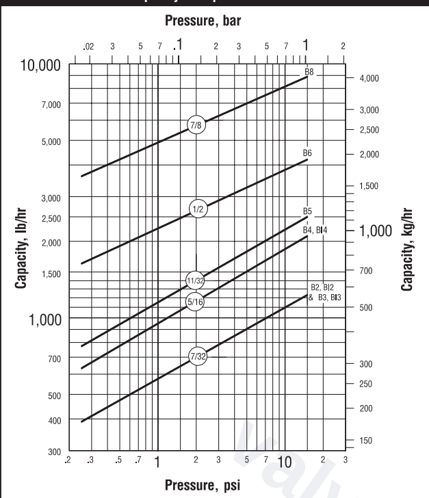
Model B & BI Series Capacity—15 psi
