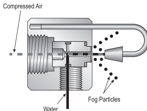
Figure 157-2. Fogger Head
