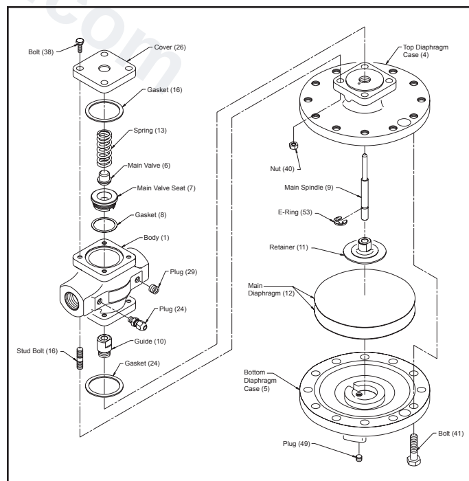
Figure 5-2. OB-2000 Main Valve
