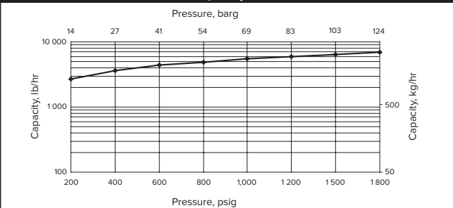
Model SH-1700 Cold Water Capacity
