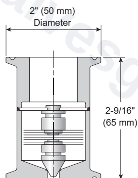
Model TC-S Sealed 1" (25 mm) Sanitary End Connections
