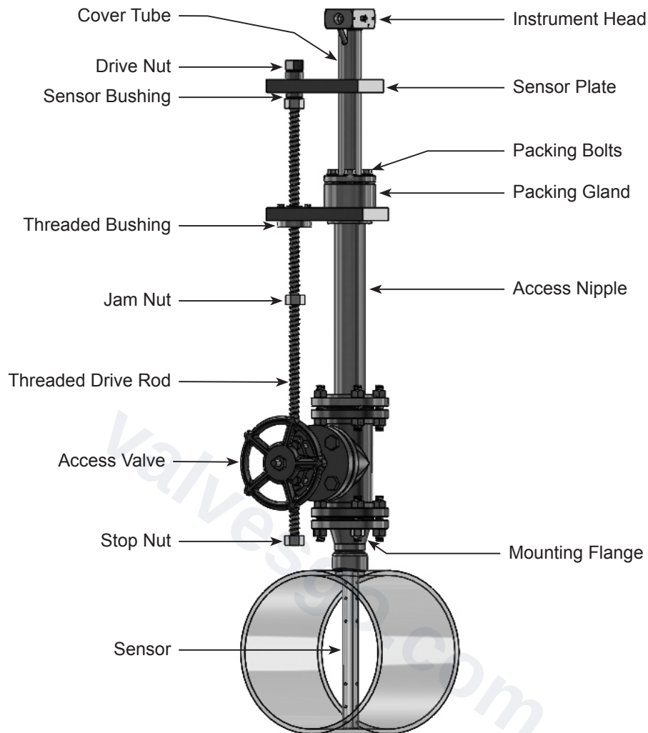
Figure 8. Installed V400S (Single Rod)
