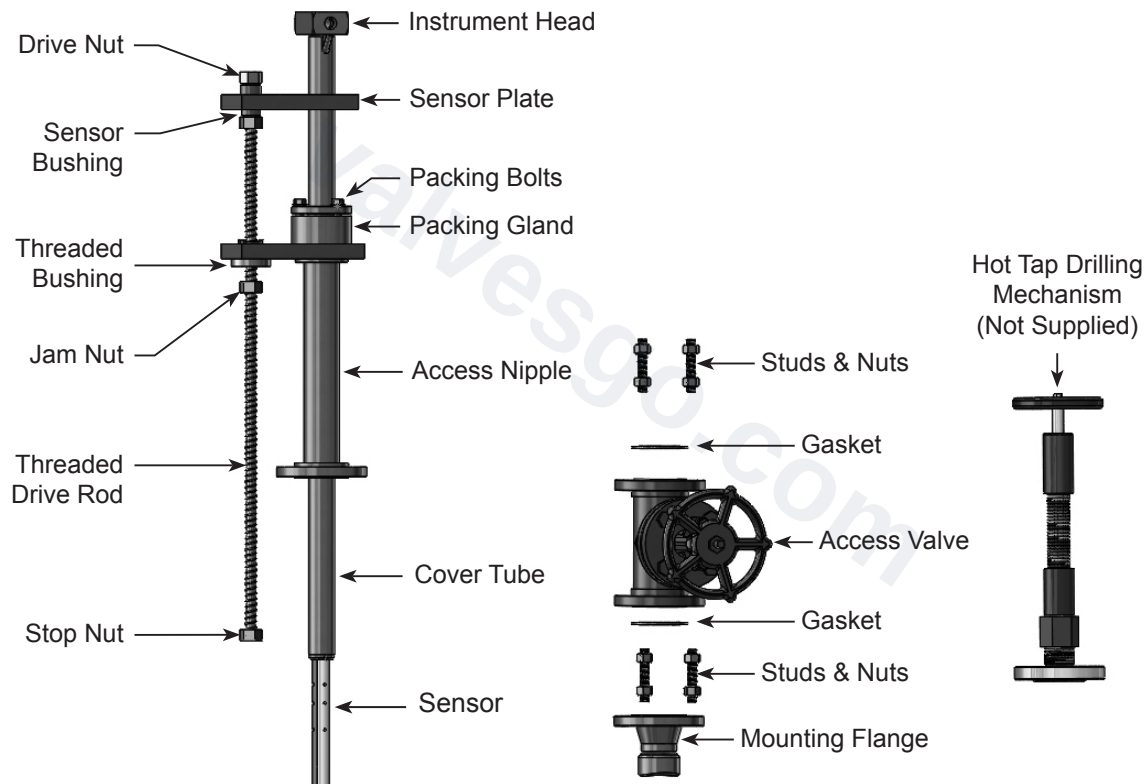
Figure 2. Verabar® Model V400S (Single Rod)
