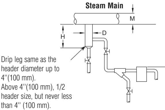
Figure 2. Trap Draining Drip Leg on Steam Main
