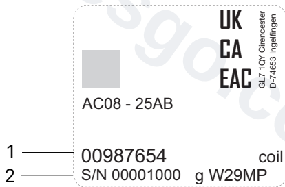
Fig. 2: Description of laser engraving on solenoid AC08
