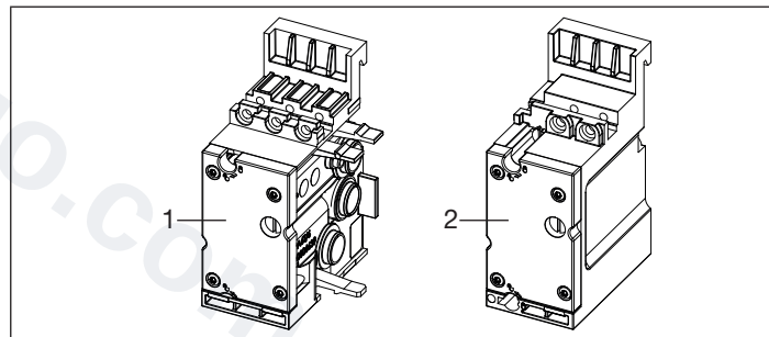
Fig. 6: Connection modules type 8640
