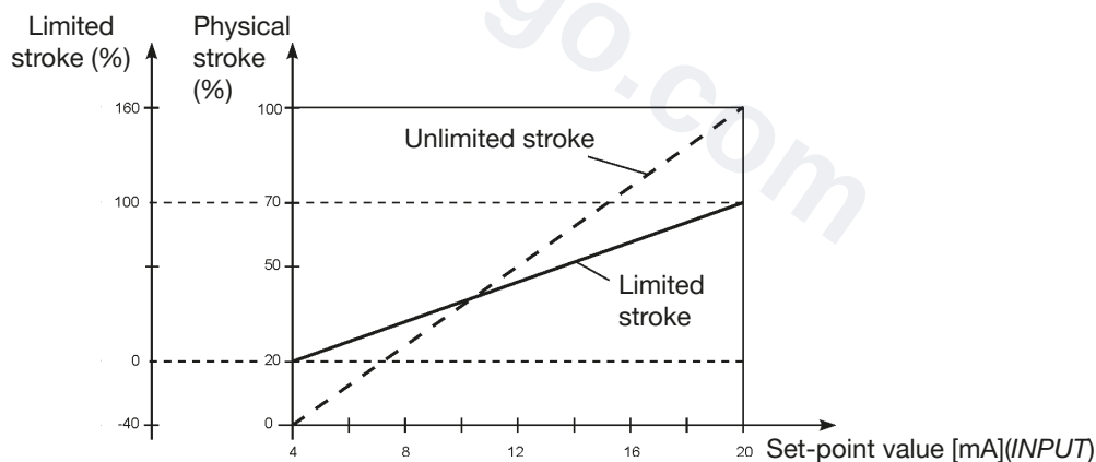
Fig. 24: Diaphragm X.LIMIT
