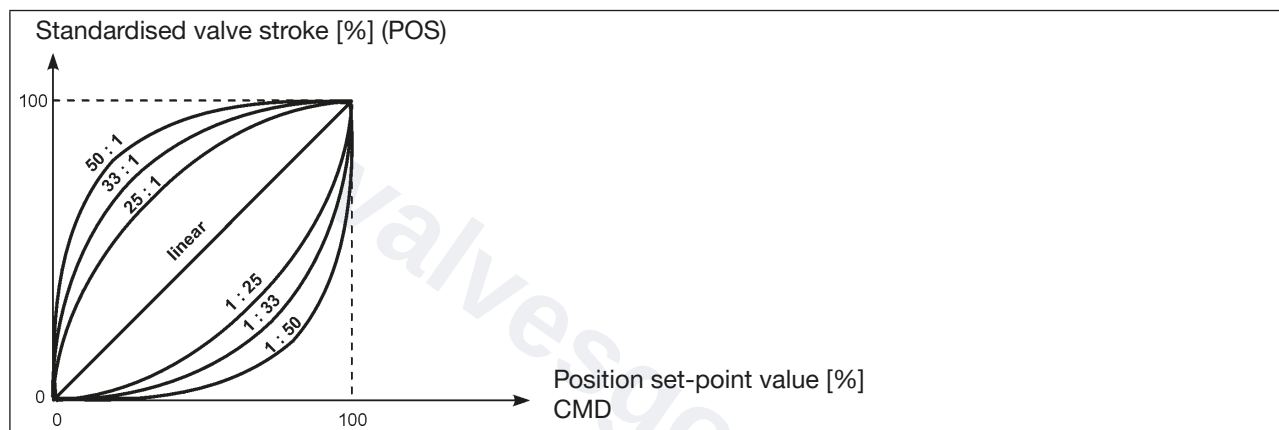
Fig. 25: Characteristics
