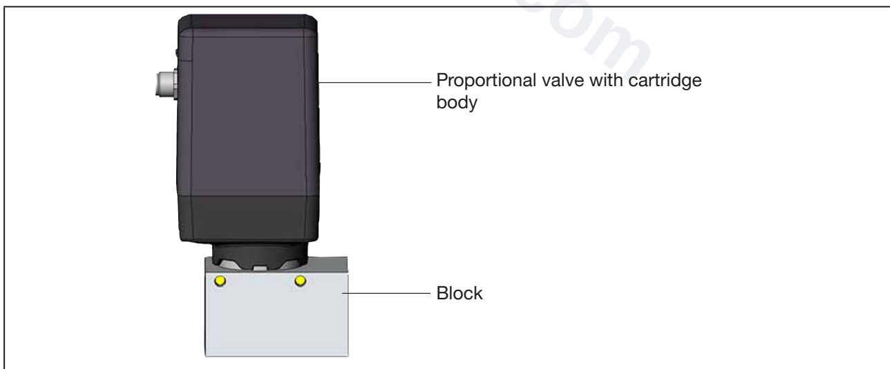
Fig. 13: Installed proportional valve with cartridge body
