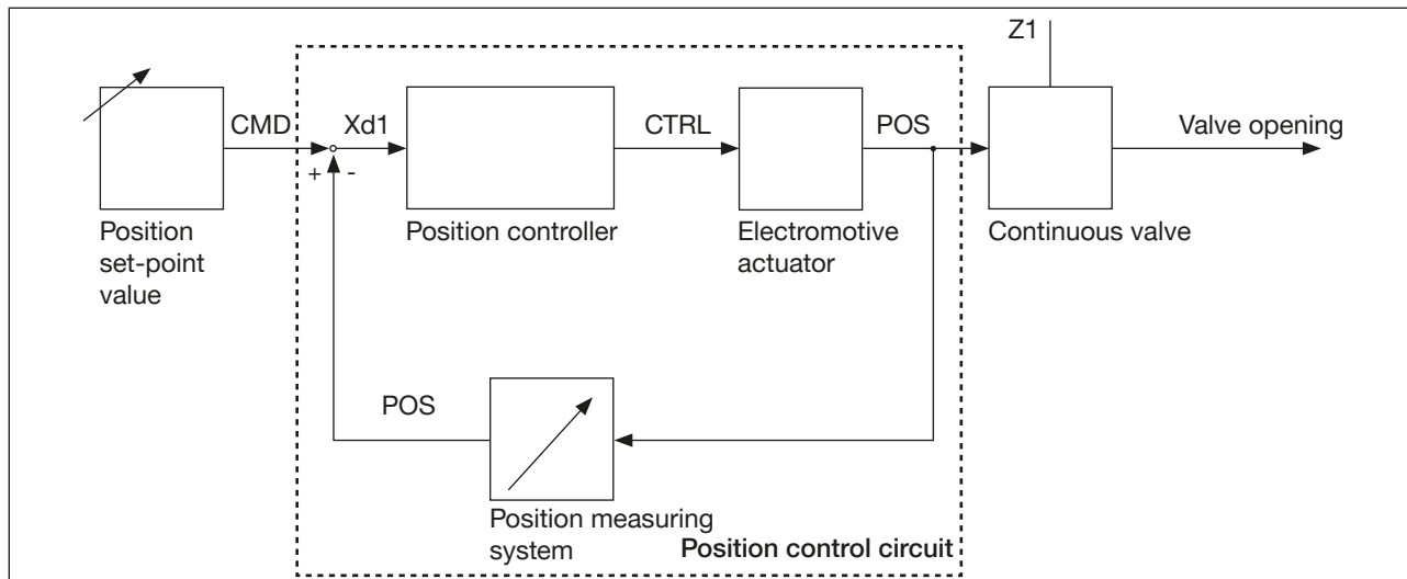
Fig. 3: Signal flow diagram position controller
