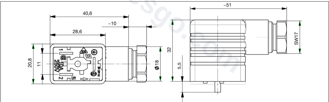
Fig. 10: Type 2516 cable plug, dimensions
