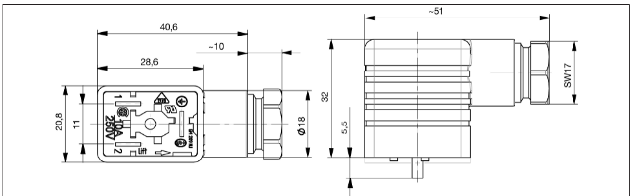
Fig. 8: Type 2507 cable plug dimensions
