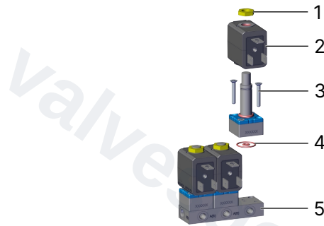
Fig. 1: Installation of devices with flange connection
