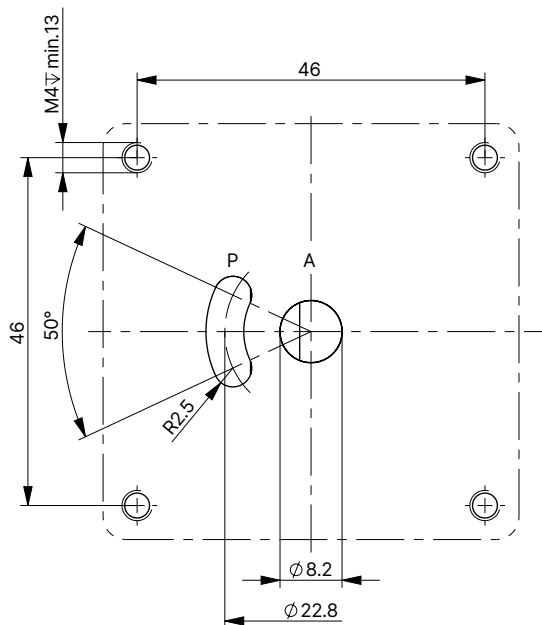
Connection contour FK14 DN 8
