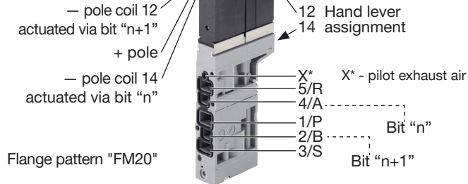
Fig. 11: Position of the connections, 2x3/2-way valve Type 6524
