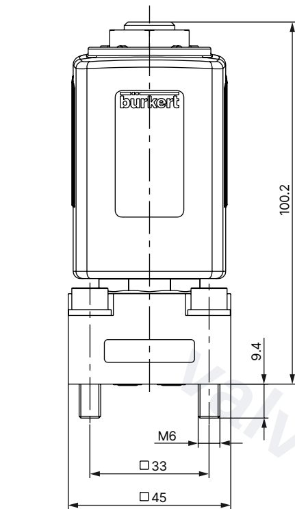
Connection outline
