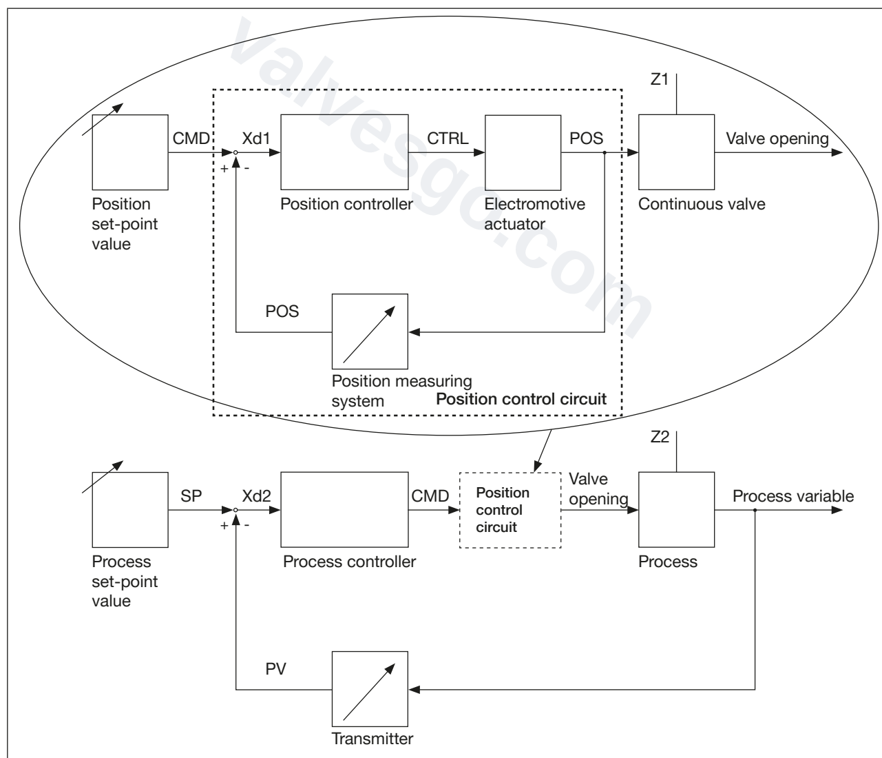
Fig. 4: Signal flow diagram process controller
