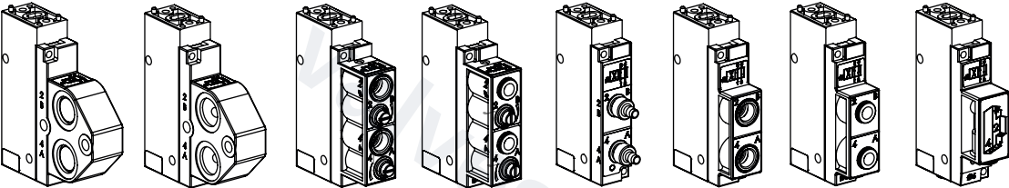
Namur Namur for throttle screws Variant B G 1/8 or NPT 1/8 Variant B Plug-in coupling Ø6 mm Variant D Variant E Variant F Variant C (code AF07)
