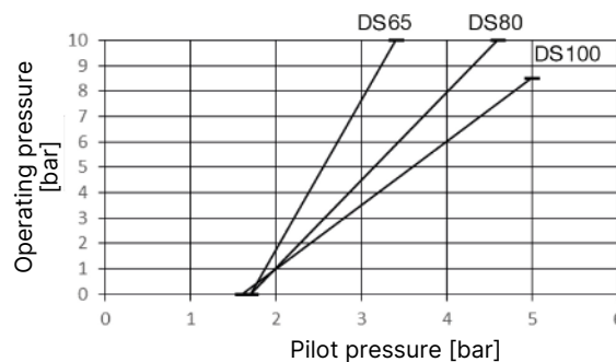
Fig. 17: Control function B, diaphragm material EPDM, FKM, actuator size 225 (L)
