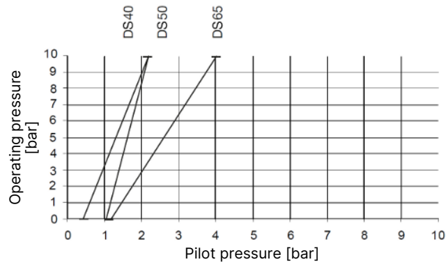
Fig. 29: Control function I, diaphragm material EPDM, FKM, actuator size 130 (P)
