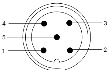
M12 circular plug, 5-pin
