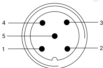
M12 circular plug, 5-pin, Port Class A
