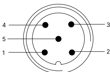
M12 circular plug, 5-pin, Port Class B
