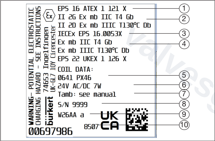
Fig. 1: Description of the type label for explosion-risk areas (example)
