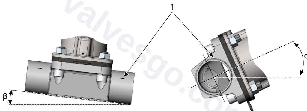
Fig. 34: Installation position for self-draining
