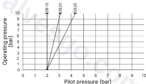
Fig. 27: Control function I, diaphragm material EPDM, FKM, actuator size 70 (M)
