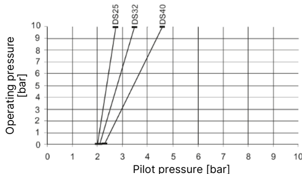
Fig. 28: Control function I, diaphragm material EPDM, FKM, actuator size 90 (N)
