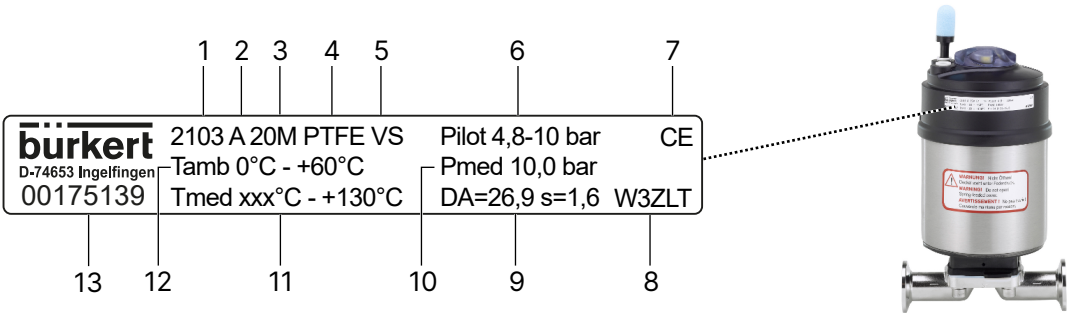
Fig. 4: Description of the type label (example)
