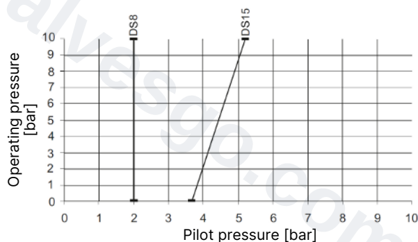
Fig. 30: Control function I, diaphragm material PTFE, advanced PTFE, GYLON®, actuator size 50 (D)
