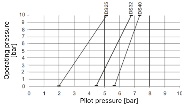
Fig. 21: Control function B, diaphragm material PTFE, advanced PTFE, GYLON®, actuator size 90 (N)
