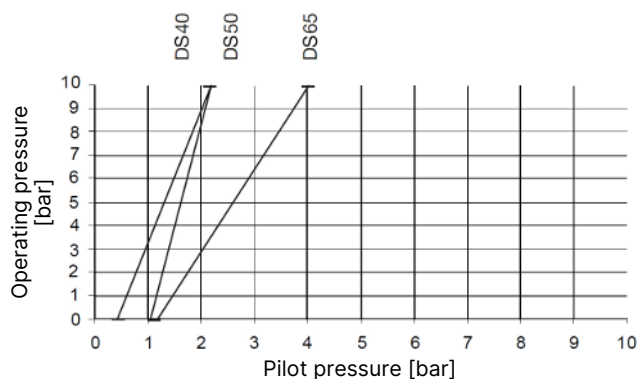
Fig. 29: Control function I, diaphragm material EPDM, FKM, actuator size 130 (P)
