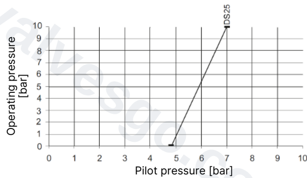
Fig. 22: Control valve, control function B, diaphragm material PTFE, advanced PTFE, GYLON®, actuator size 90 (N)
