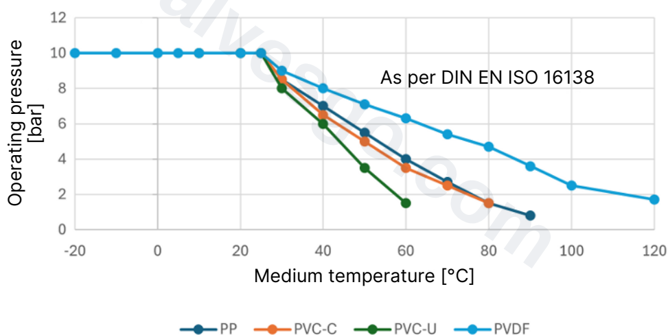
Fig. 9: Pressure temperature diagram for plastic valve body
