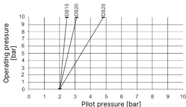
Fig. 31: Control function I, diaphragm material PTFE, advanced PTFE, GYLON®, actuator size 70 (M)
