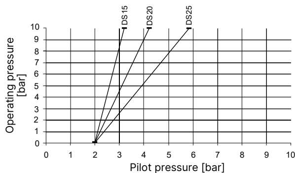
Fig. 11: Control function B, diaphragm material EPDM, FKM, actuator size 70 (M)
