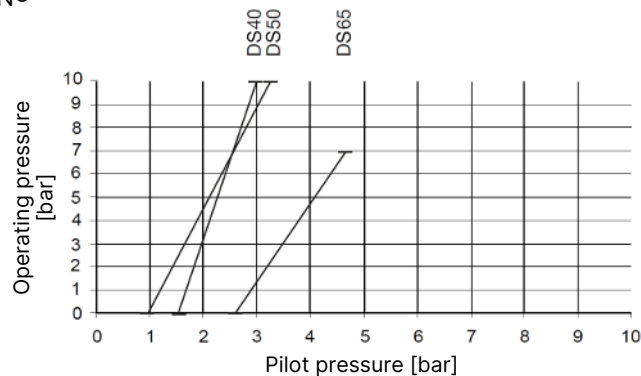
Fig. 23: Control function B, diaphragm material PTFE, advanced PTFE, GYLON®, actuator size 130 (P)
