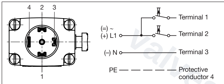
Fig. 1: Circuit diagram connection of pulse valve
