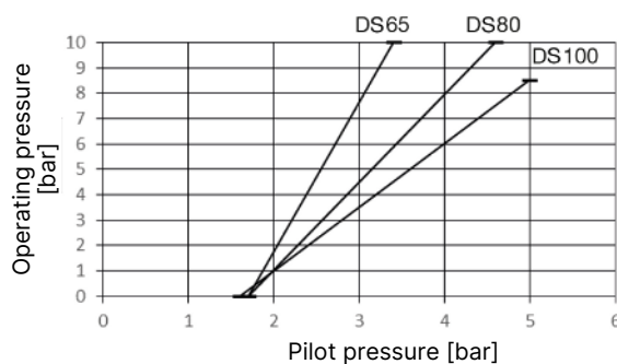
Fig. 14: Control function B, diaphragm material EPDM, FKM, actuator size 225 (L)
