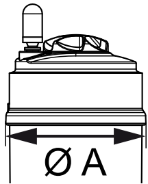
Fig. 6: Determination of actuator size based on the outer diameter A of the actuator cover
