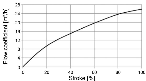
Fig. 24: Actuator size 70 (M), flow characteristic DN32
