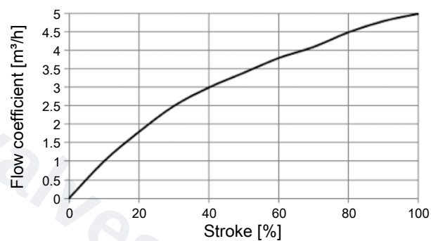
Fig. 21: Actuator size 70 (M), flow characteristic DN15
