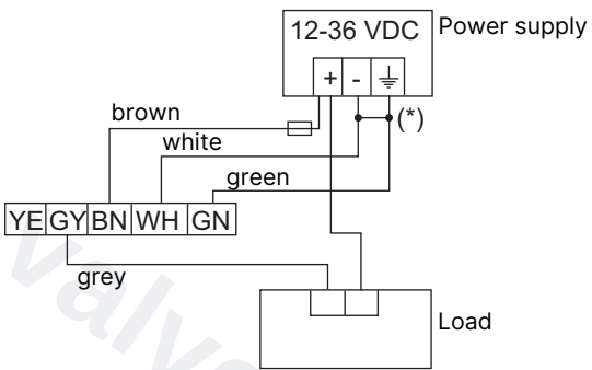
Fig. 14: NPN wiring (default) of the pulse output of a version with cable gland
