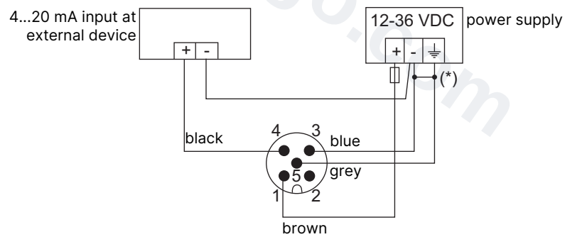
Fig. 13: Wiring the current output in sourcing mode on a version with M12 fixed connector.
