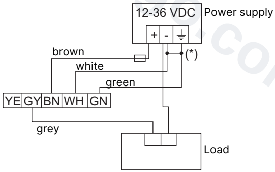
Fig. 15: PNP wiring of the pulse output of a version with cable gland
