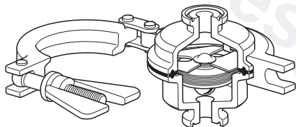
Sanitary clamp ended variant
