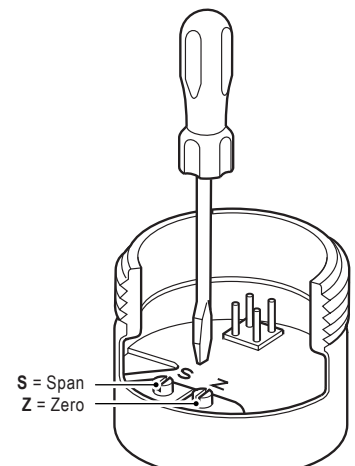
Fig. 3 Calibration - Location of span and zero potentiometers
