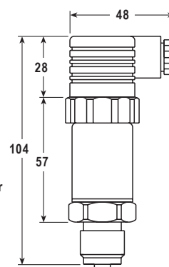
Fig. 1 EL2600 pressure transmitter
