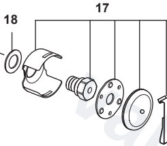
Capsule air vent assembly
