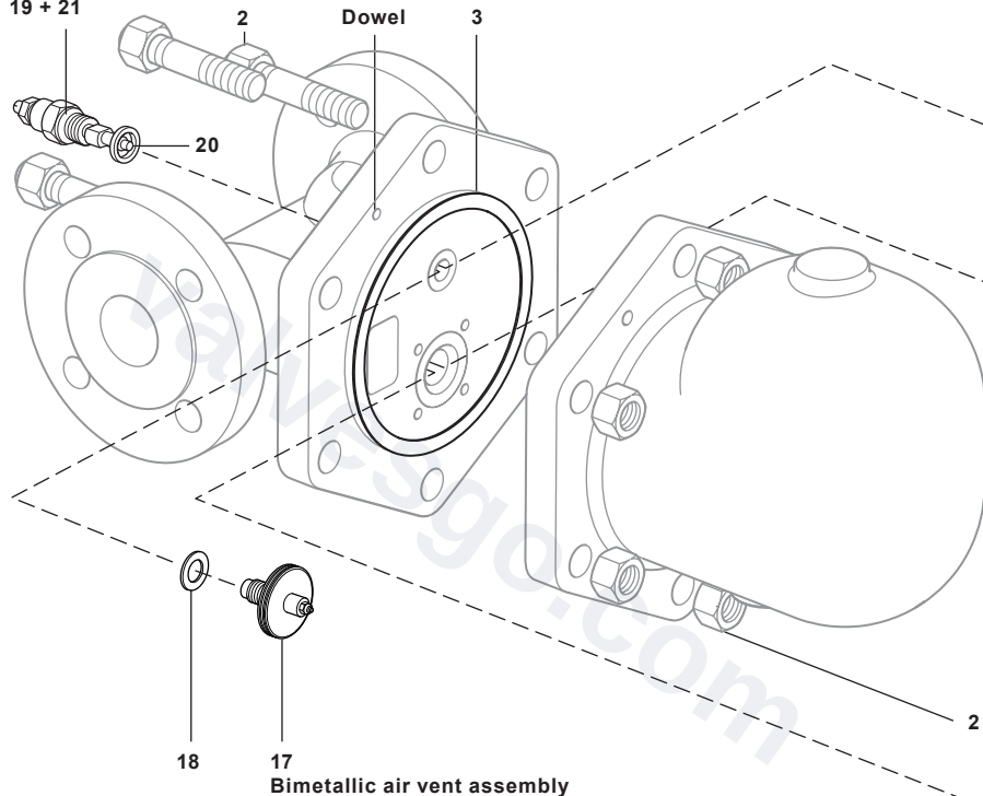
Steam lock release assembly 19 + 21
