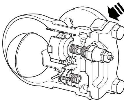
Fig. 2 FTS14-C (R-L) - Flanged
