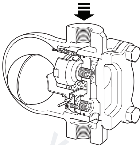
Fig. 1 FTS14X - Screwed (vertical down)
