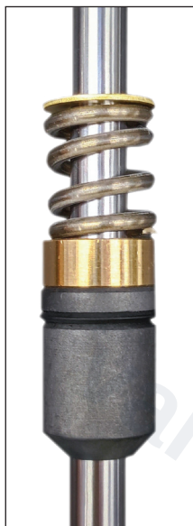
Fig. 13 Stem seal replacement kit for type PF51 Type 2 and Type 3 actuators
