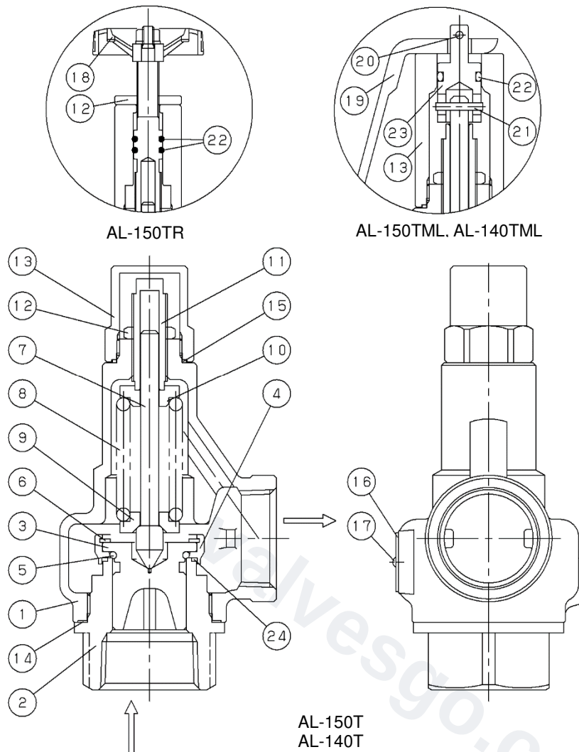
Fig.2 Structure
