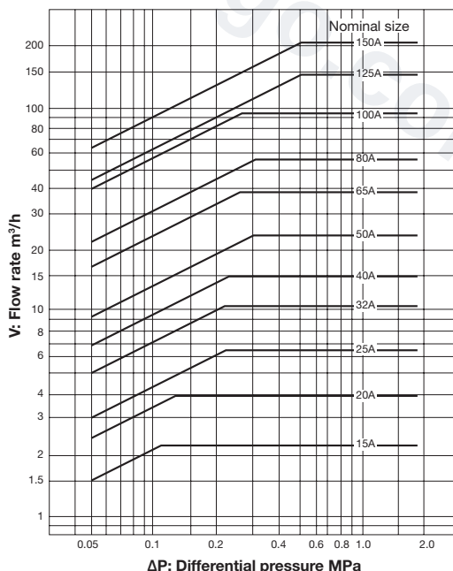
Nominal Sizes Selection Chart (For Water)
