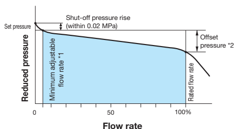
Flow Characteristic Chart
