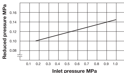
Pressure Characteristic Chart
