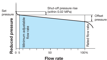
Flow Characteristic Chart
