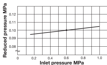
Pressure Characteristic Chart
