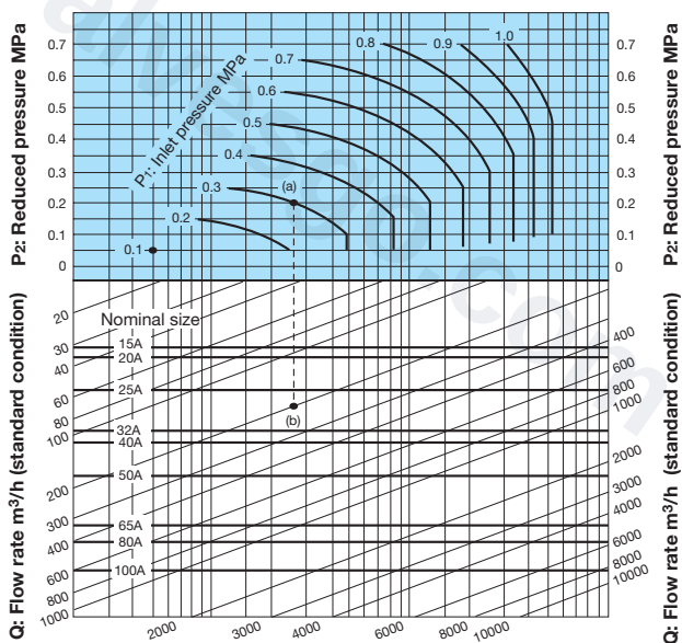
Nominal Sizes Selection Chart
