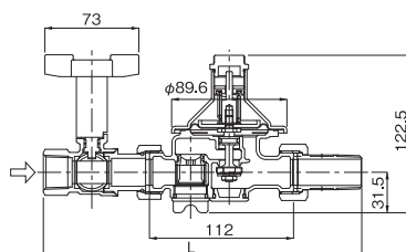
(Equipped with stop valve)
