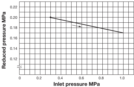
Pressure Characteristic Chart
