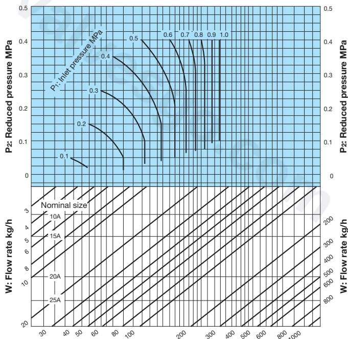
GD-6N Nominal Sizes Selection Chart(For Steam)
