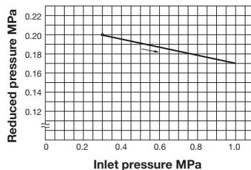
Pressure Characteristic Chart
