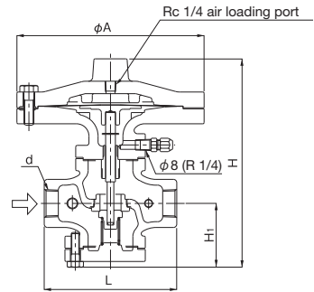
Screwed type
