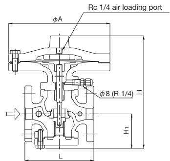
Flanged type
