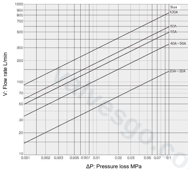
Fig. 1 Pressure loss chart
