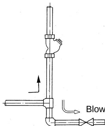
Fig. 2 Vertical piping
