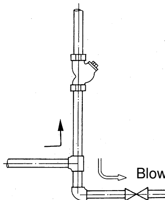
Fig. 2 Vertical piping
