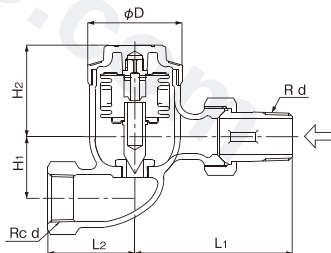
TS-1S (直线型)
