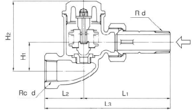
TS-3S <Straight type>
