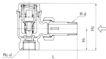
TS-4A <Angle type>
