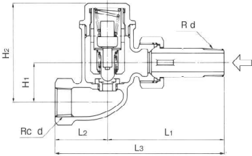
TS-4S <Straight type>
